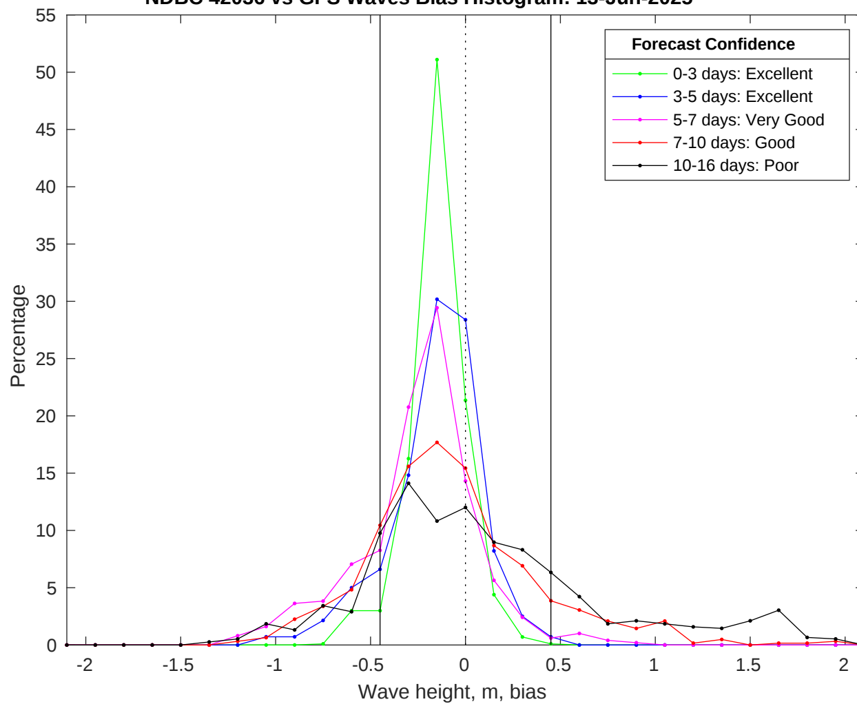
NDBC 42036 vs GFS Waves Bias Histogram: 13-Jun-2025
