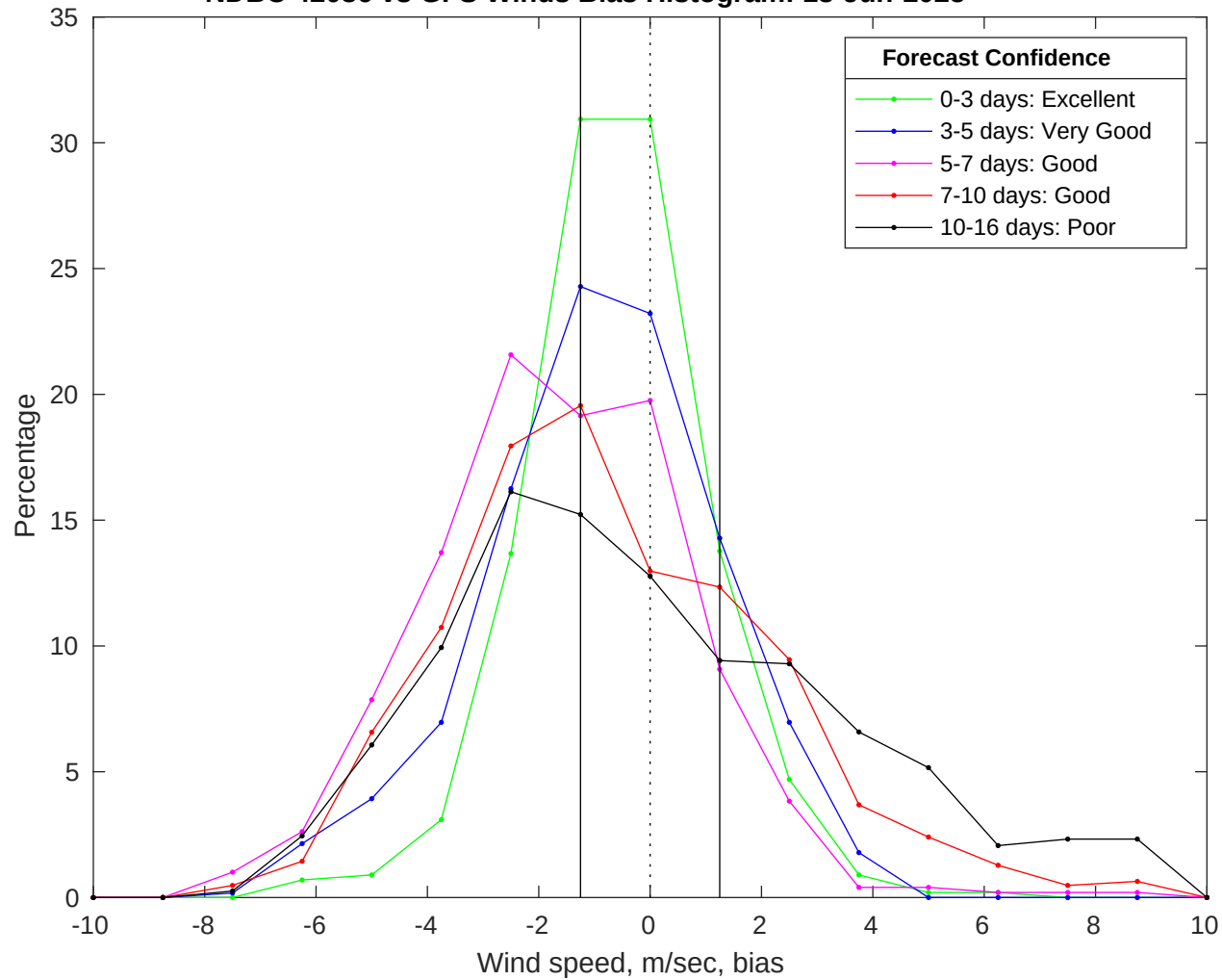
NDBC 42036 vs GFS Winds Bias Histogram: 13-Jun-2025
