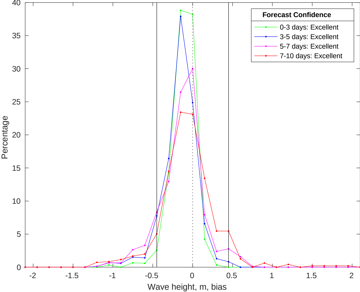
NDBC 42040 vs CMEMS Waves Bias Histogram: 13-Jun-2025
