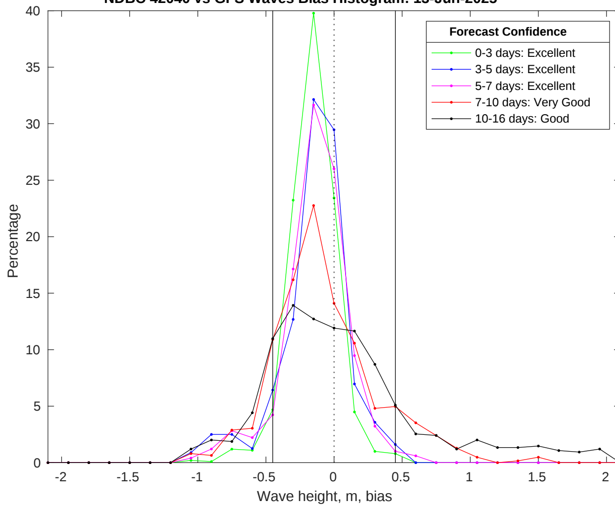
NDBC 42040 vs GFS Waves Bias Histogram: 13-Jun-2025
