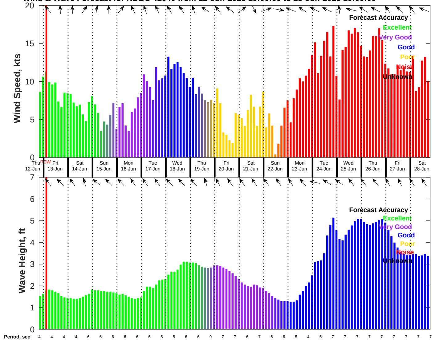
Wind & Wave Forecast for NDBC 42040 from 12-Jun-2025 19:00:00 to 28-Jun-2025 19:00:00
