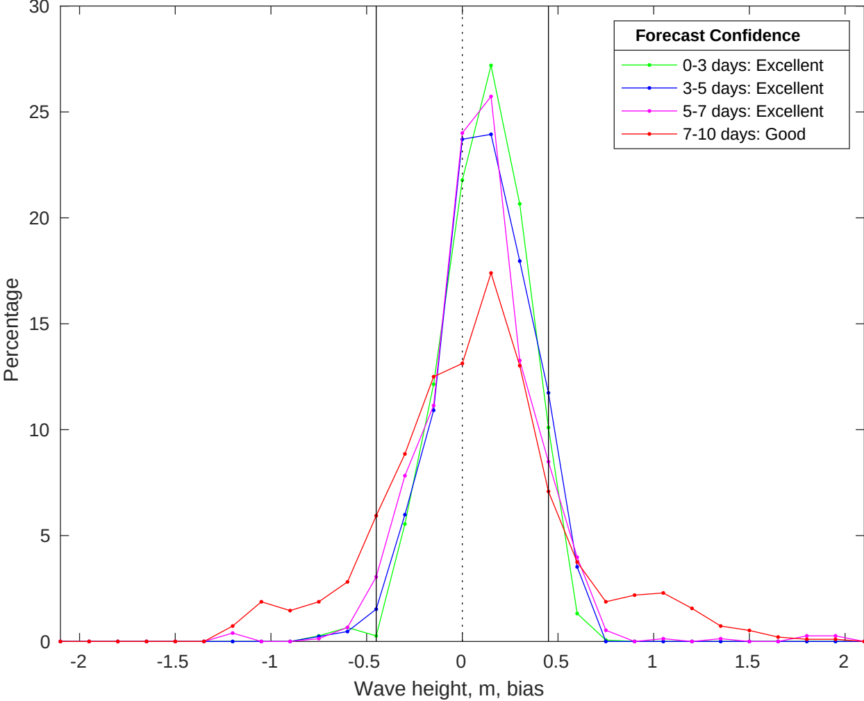
NDBC 46011 vs CMEMS Waves Bias Histogram: 13-Jun-2025
