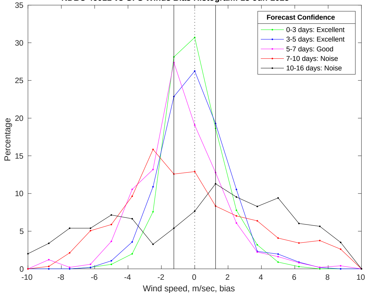
NDBC 46011 vs GFS Winds Bias Histogram: 13-Jun-2025
