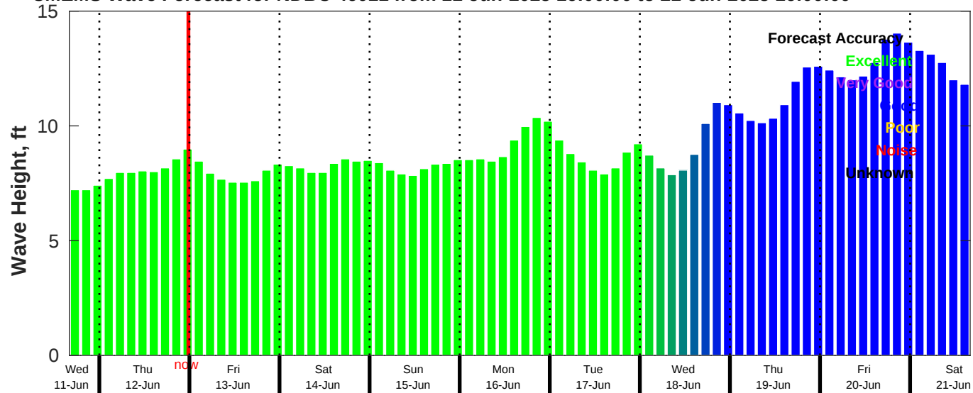
CMEMS Wave Forecast for NDBC 46011 from 11-Jun-2025 16:00:00 to 21-Jun-2025 16:00:00
