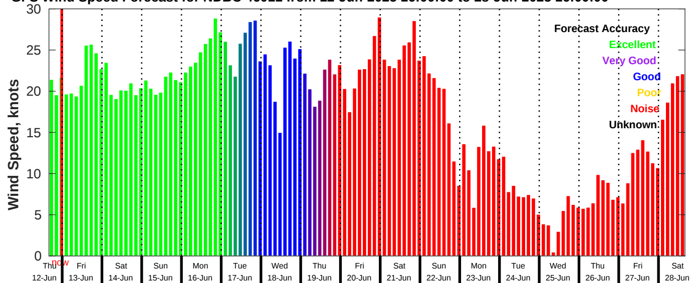
GFS Wind Speed Forecast for NDBC 46011 from 12-Jun-2025 16:00:00 to 28-Jun-2025 16:00:00
