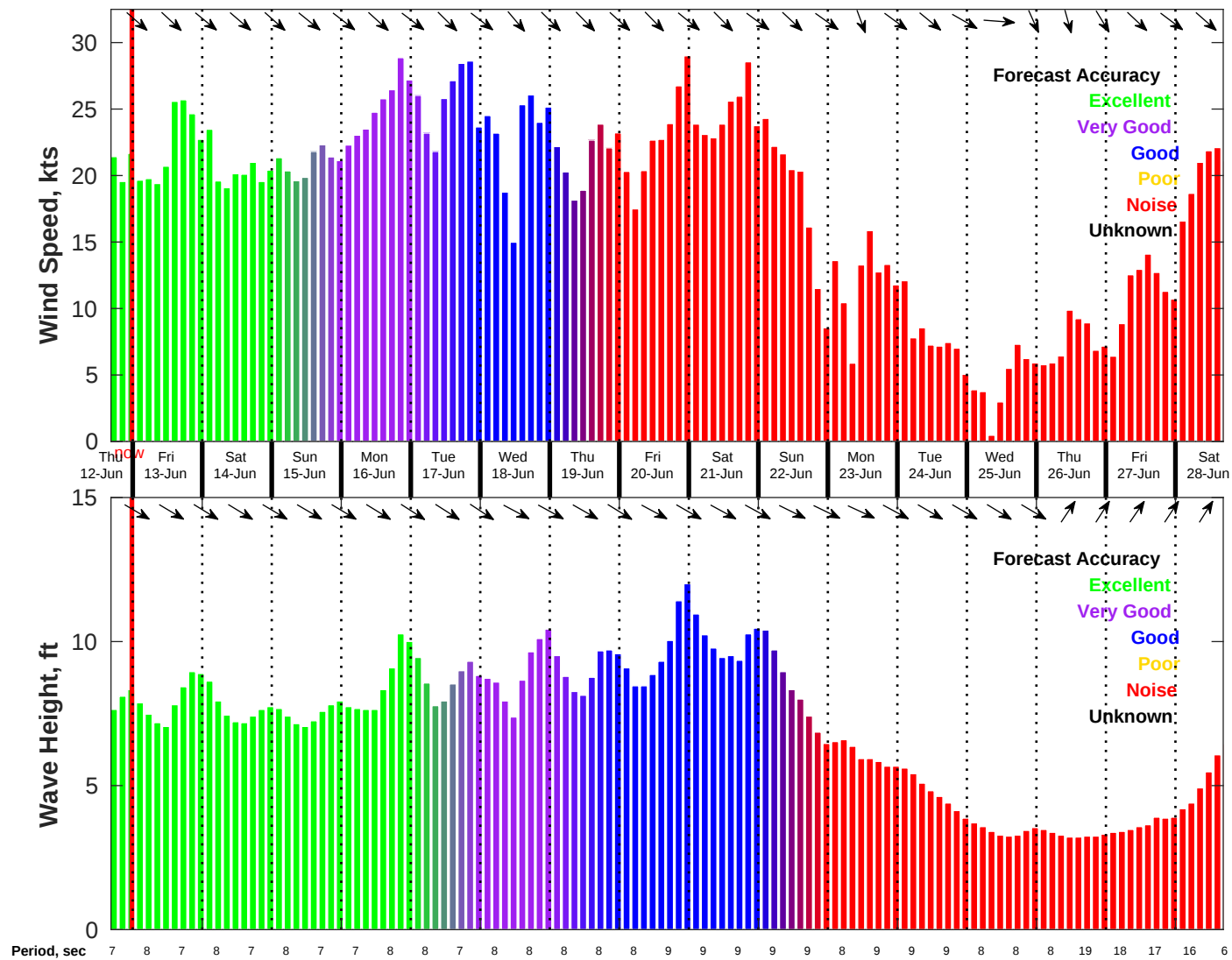
Wind & Wave Forecast for NDBC 46011 from 12-Jun-2025 16:00:00 to 28-Jun-2025 16:00:00
