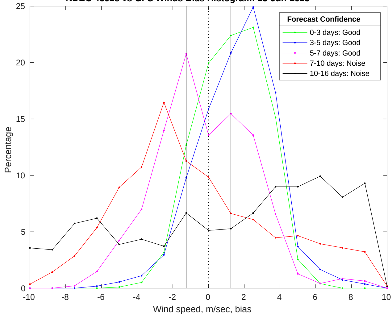
NDBC 46028 vs GFS Winds Bias Histogram: 13-Jun-2025
