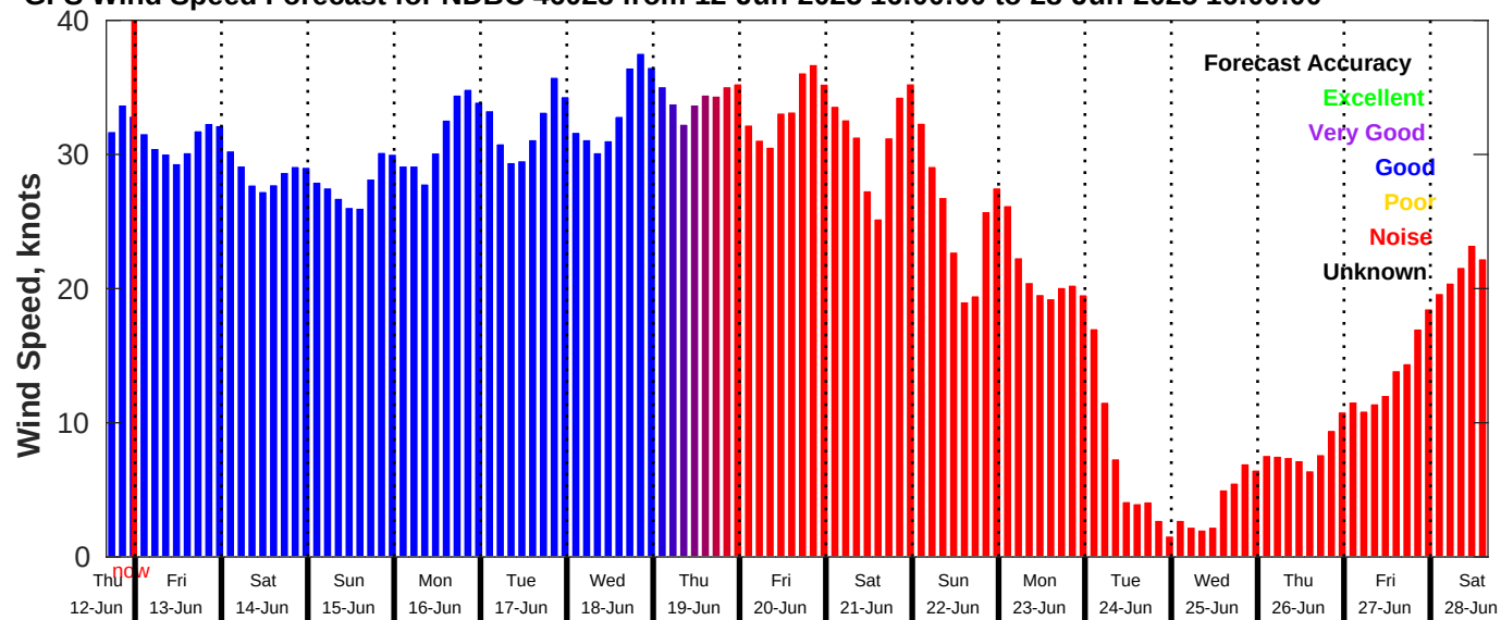
GFS Wind Speed Forecast for NDBC 46028 from 12-Jun-2025 16:00:00 to 28-Jun-2025 16:00:00
