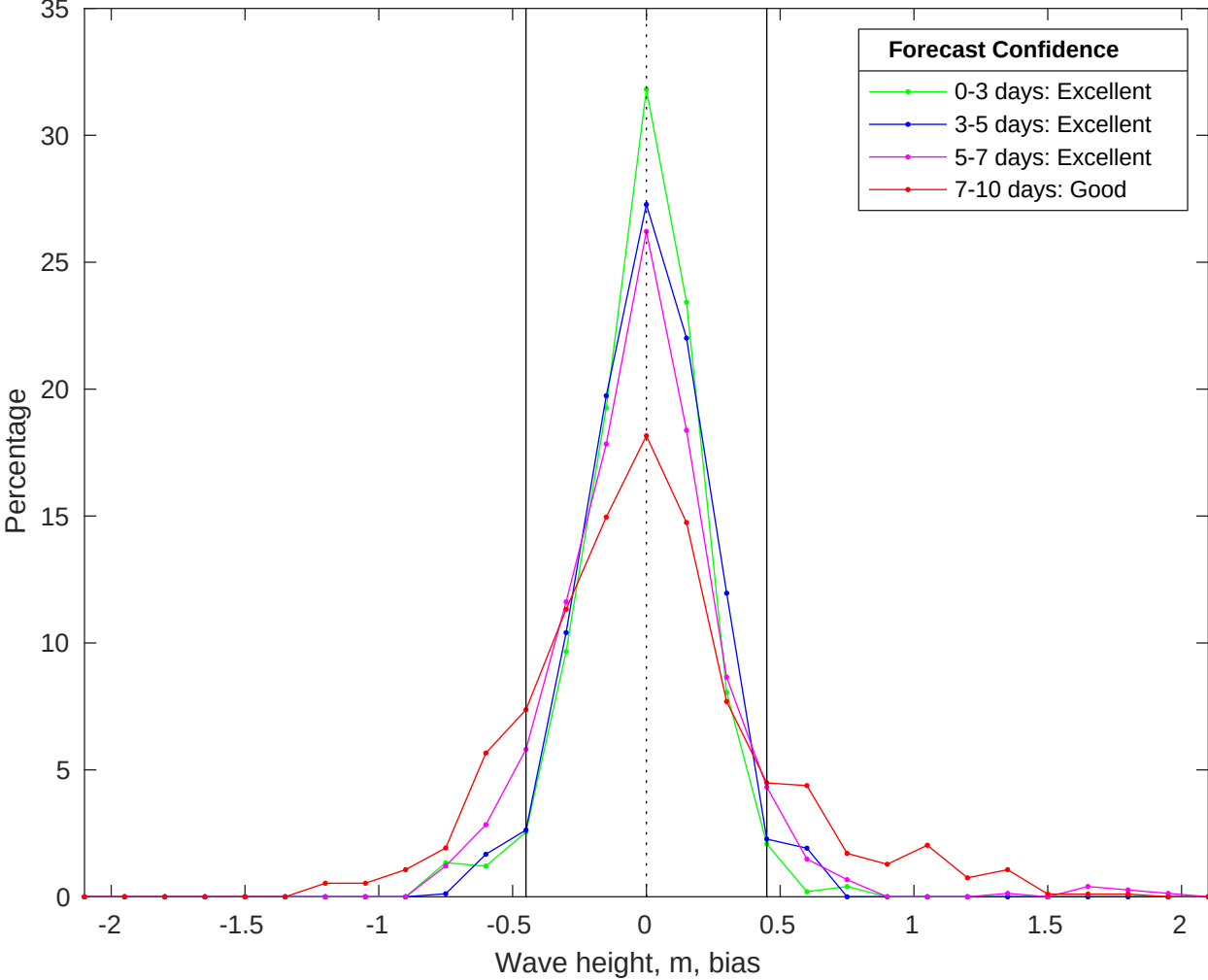
NDBC 46054 vs CMEMS Waves Bias Histogram: 13-Jun-2025
