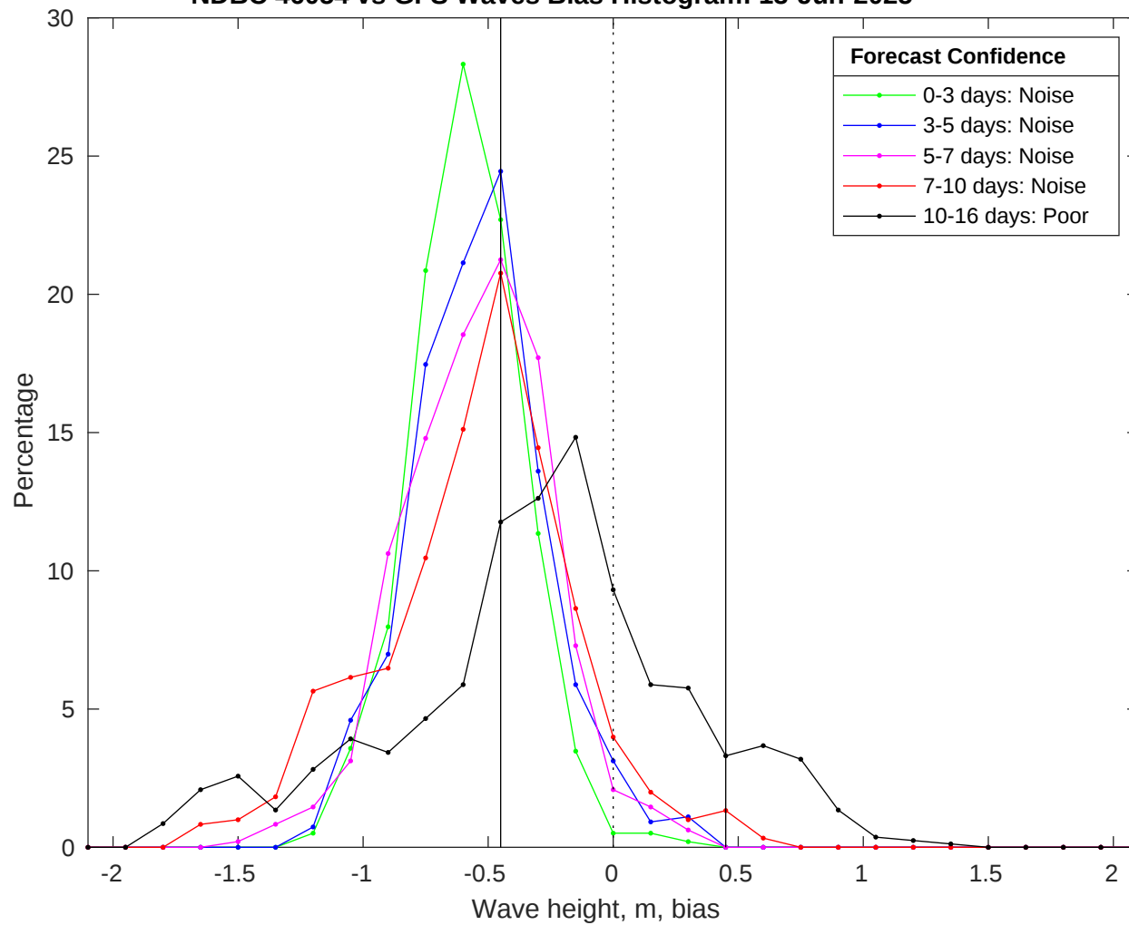
NDBC 46054 vs GFS Waves Bias Histogram: 13-Jun-2025
