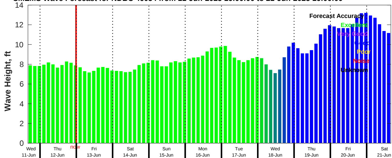
CMEMS Wave Forecast for NDBC 46054 from 11-Jun-2025 16:00:00 to 21-Jun-2025 16:00:00
