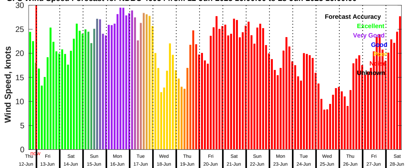
GFS Wind Speed Forecast for NDBC 46054 from 12-Jun-2025 16:00:00 to 28-Jun-2025 16:00:00
