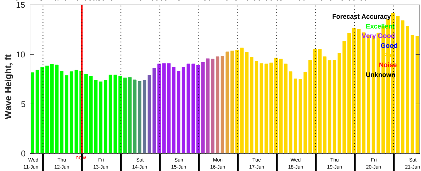
CMEMS Wave Forecast for NDBC 46069 from 11-Jun-2025 16:00:00 to 21-Jun-2025 16:00:00
