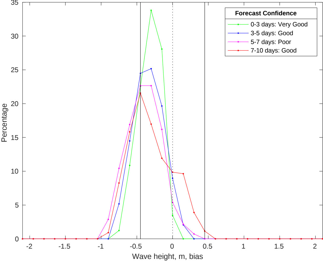
NDBC 51209 vs CMEMS Waves Bias Histogram: 13-Jun-2025
