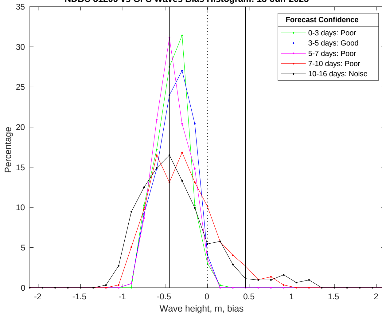
NDBC 51209 vs GFS Waves Bias Histogram: 13-Jun-2025
