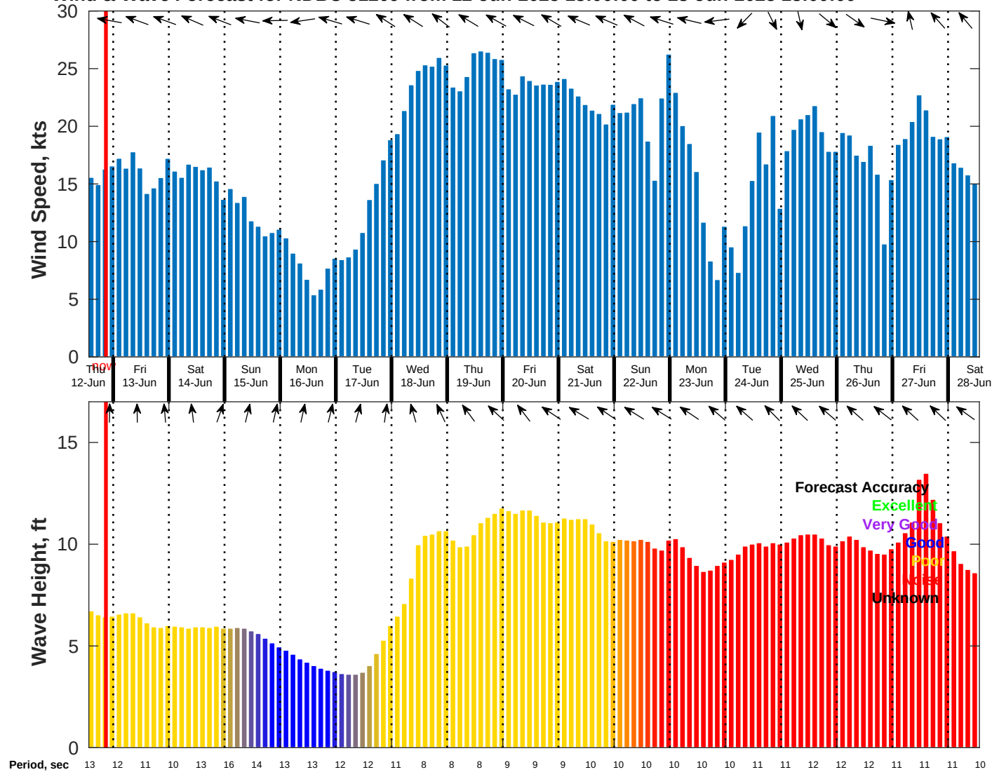
Wind & Wave Forecast for NDBC 51209 from 12-Jun-2025 13:00:00 to 28-Jun-2025 13:00:00
