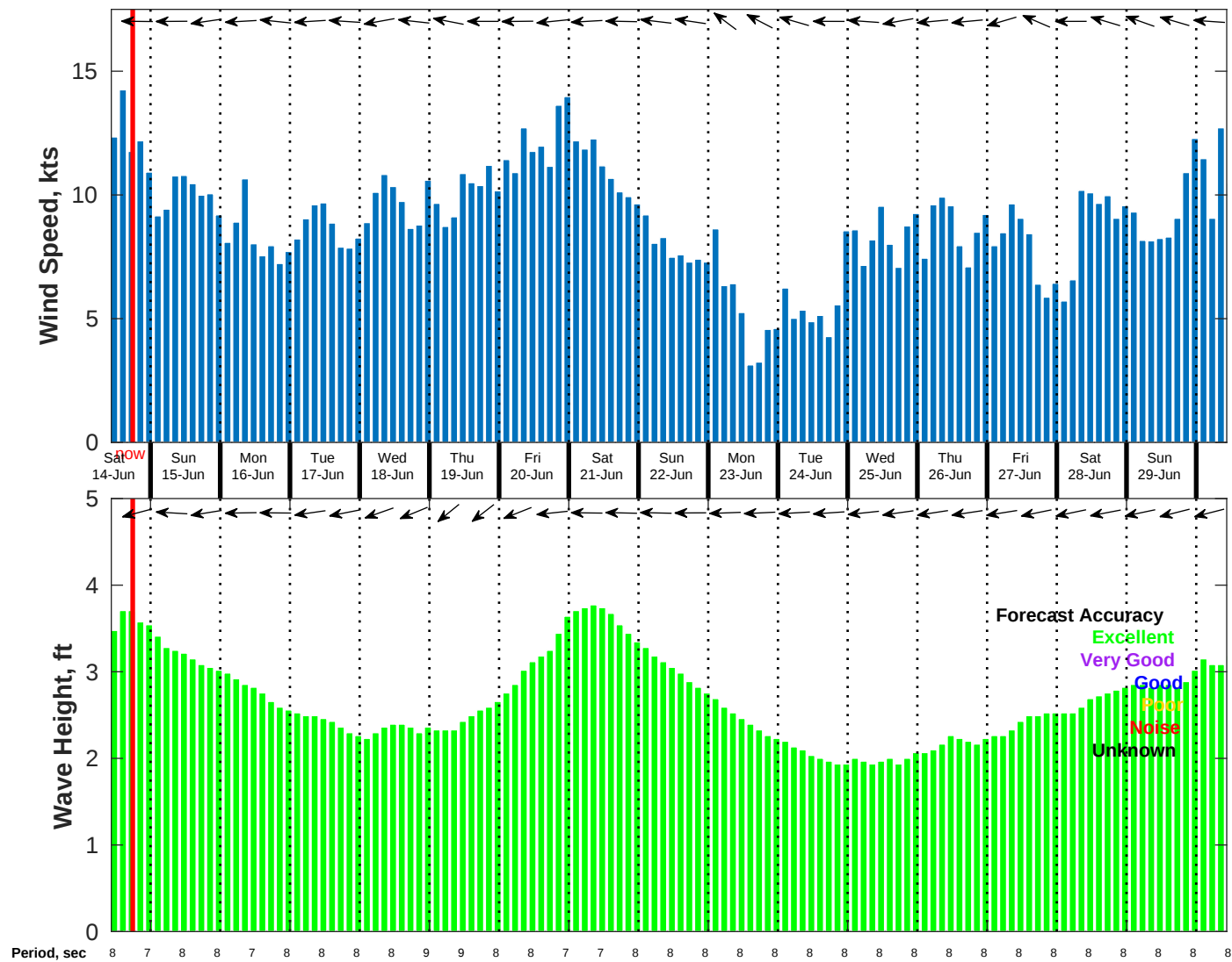
Wind & Wave Forecast for NDBC 52211 from 13-Jun-2025 10:00:00 to 29-Jun-2025 10:00:00
