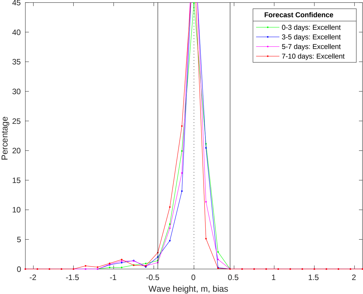
NDBC 52212 vs CMEMS Waves Bias Histogram: 13-Jun-2025
