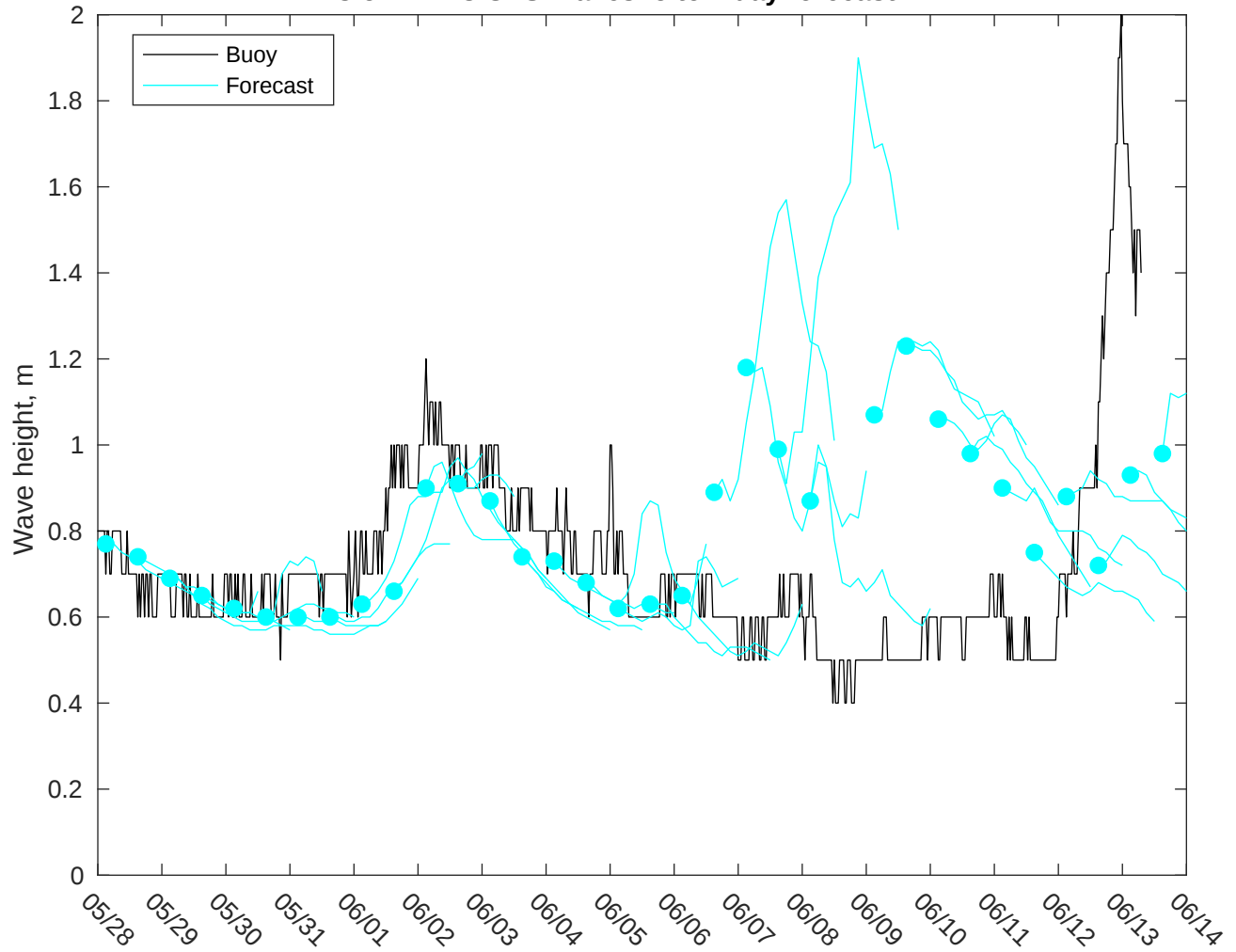
NDBC 52212 vs GFS Waves: 5 to 7 day forecast
