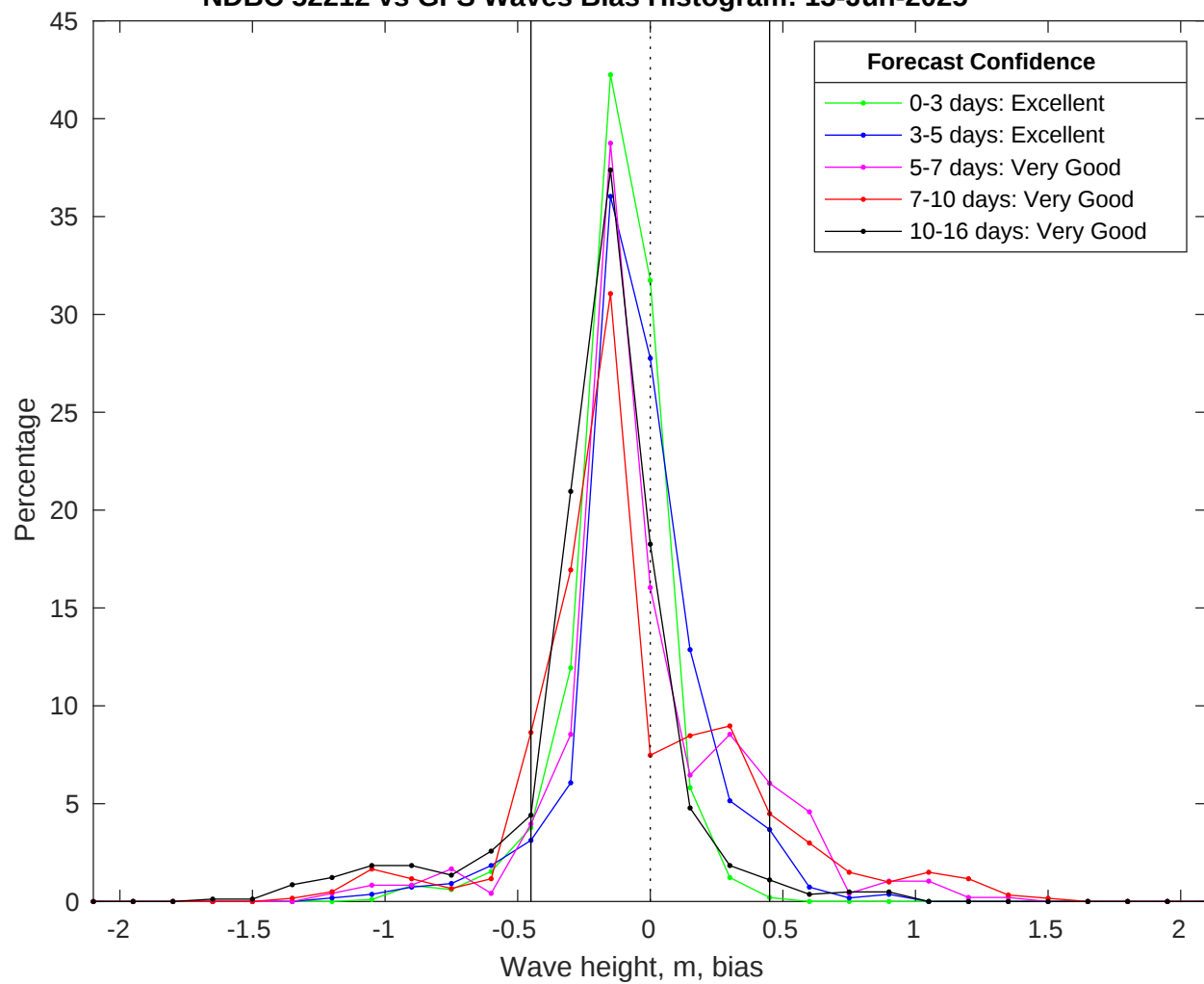
NDBC 52212 vs GFS Waves Bias Histogram: 13-Jun-2025
