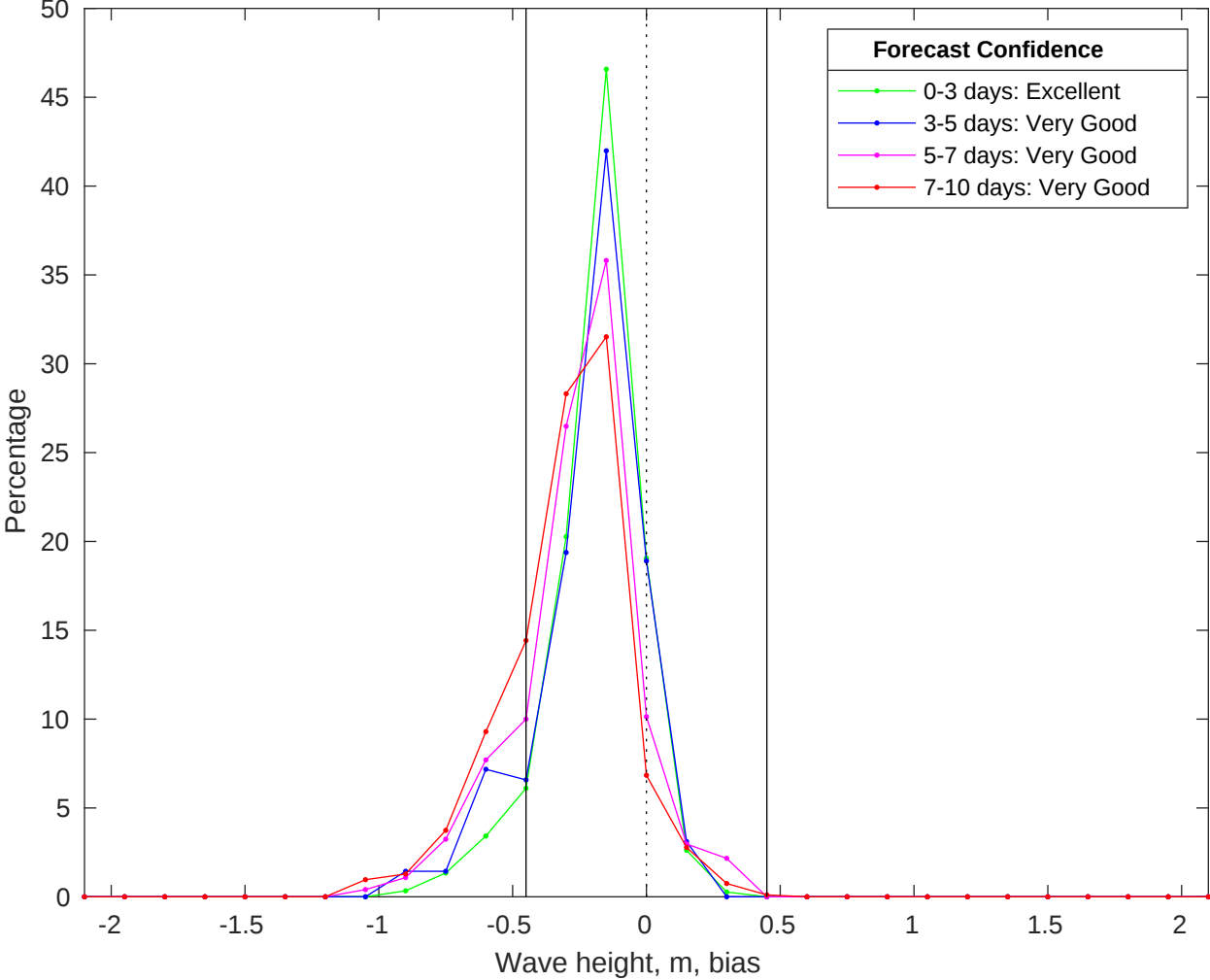
NDBC 52213 vs CMEMS Waves Bias Histogram: 13-Jun-2025
