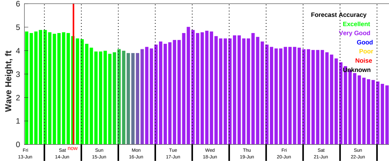
CMEMS Wave Forecast for NDBC 52213 from 12-Jun-2025 11:00:00 to 22-Jun-2025 11:00:00
