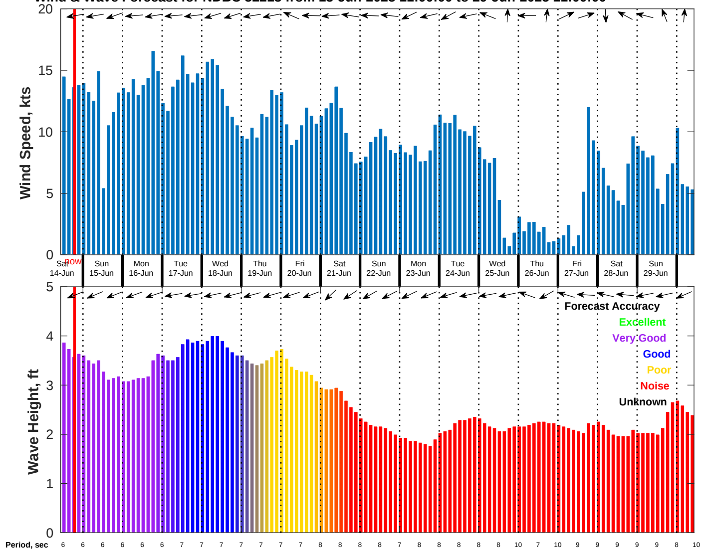
Wind & Wave Forecast for NDBC 52213 from 13-Jun-2025 11:00:00 to 29-Jun-2025 11:00:00
