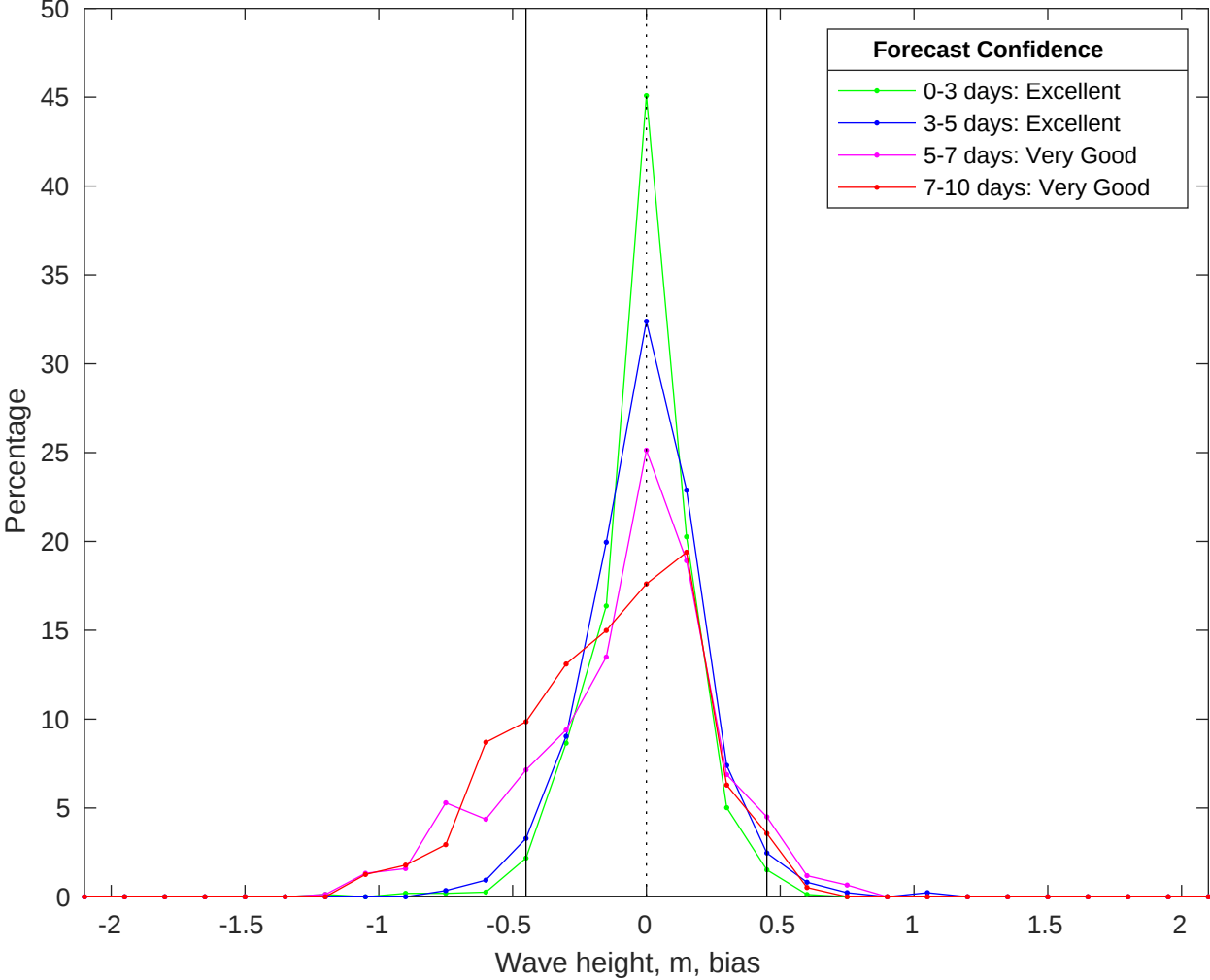
NDBC 41004 vs CMEMS Waves Bias Histogram: 14-Jun-2025
