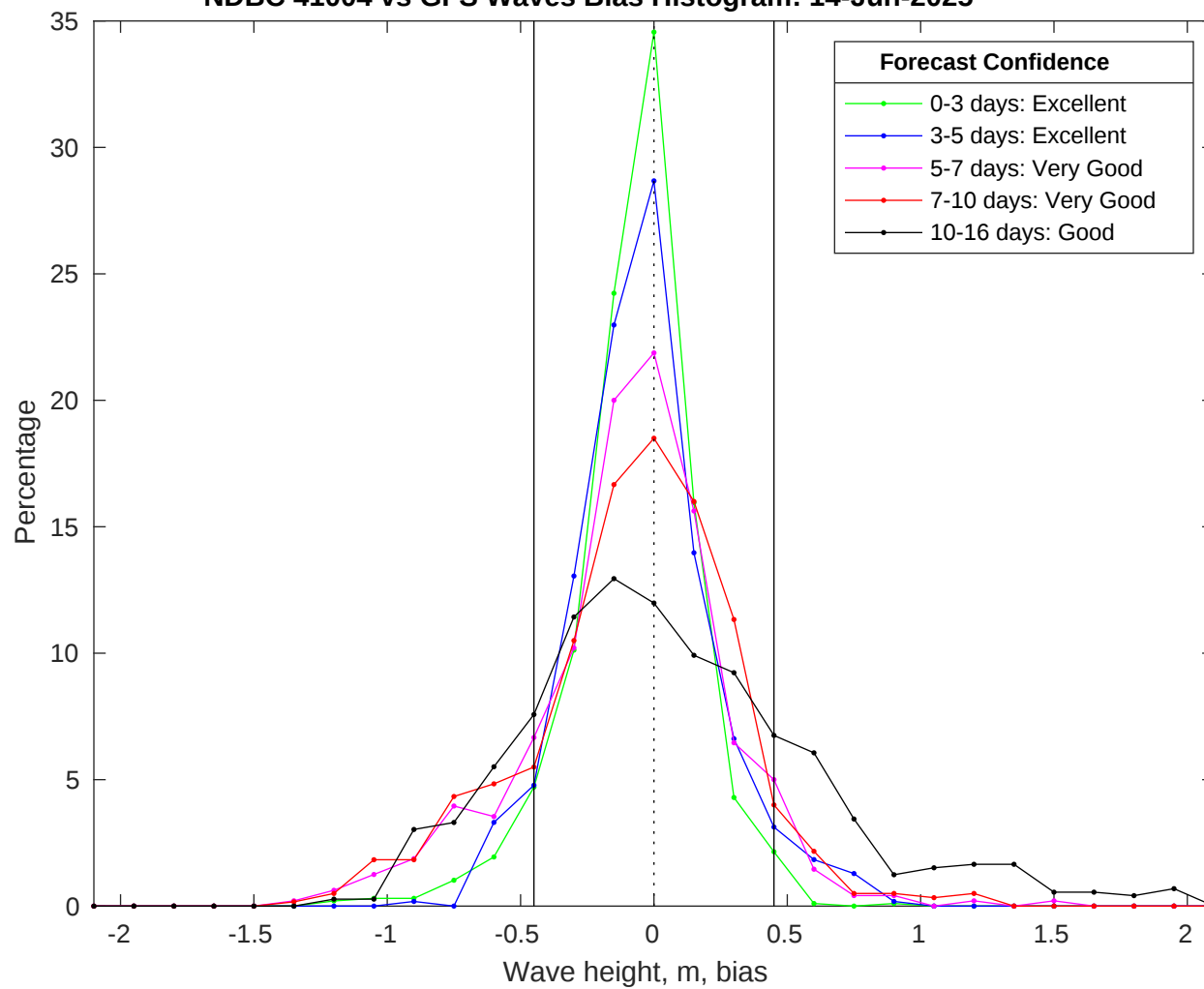
NDBC 41004 vs GFS Waves Bias Histogram: 14-Jun-2025
