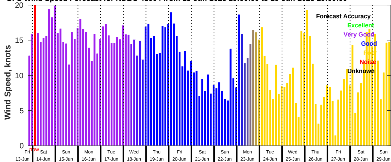
GFS Wind Speed Forecast for NDBC 41004 from 13-Jun-2025 19:00:00 to 29-Jun-2025 19:00:00
