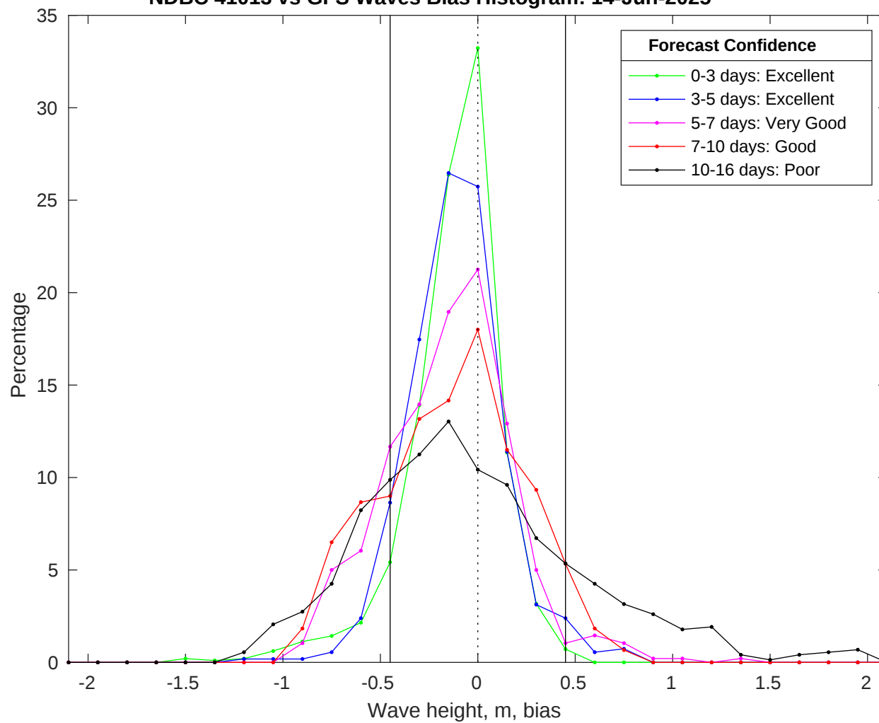
NDBC 41013 vs GFS Waves Bias Histogram: 14-Jun-2025
