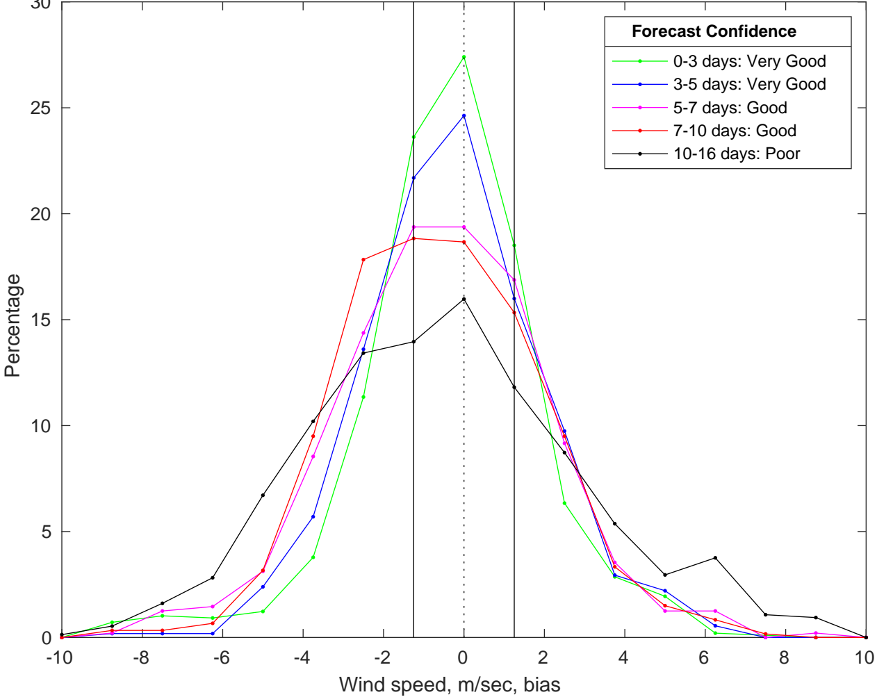
NDBC 41013 vs GFS Winds Bias Histogram: 14-Jun-2025
