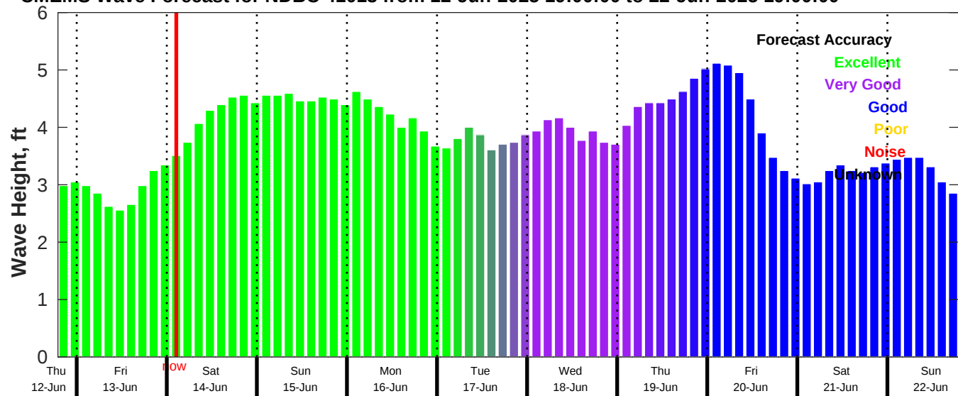
CMEMS Wave Forecast for NDBC 41013 from 12-Jun-2025 19:00:00 to 22-Jun-2025 19:00:00
