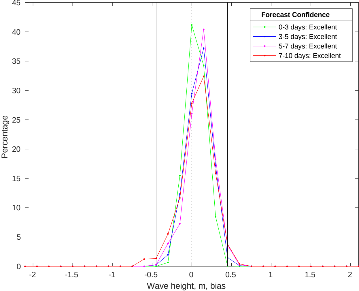
NDBC 41040 vs CMEMS Waves Bias Histogram: 14-Jun-2025
