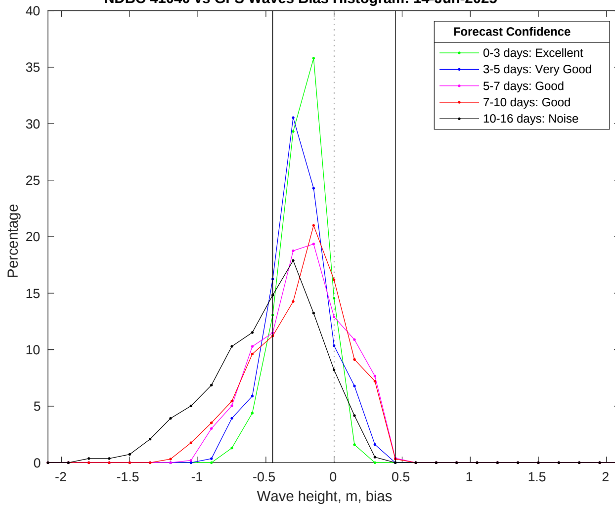
NDBC 41040 vs GFS Waves Bias Histogram: 14-Jun-2025
