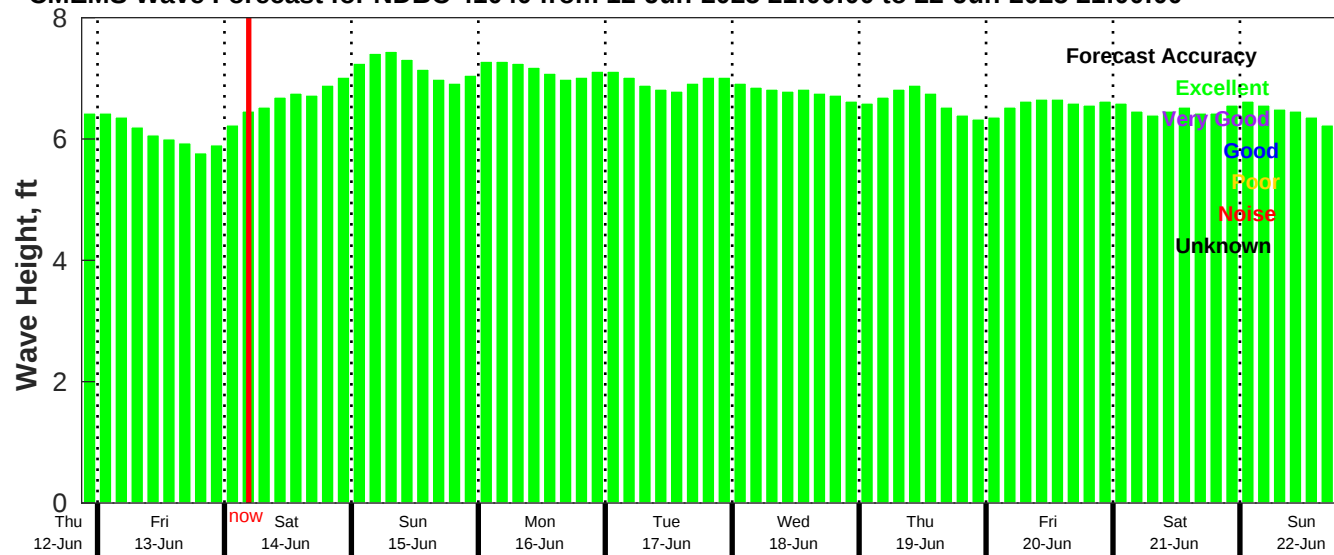
CMEMS Wave Forecast for NDBC 41040 from 12-Jun-2025 21:00:00 to 22-Jun-2025 21:00:00
