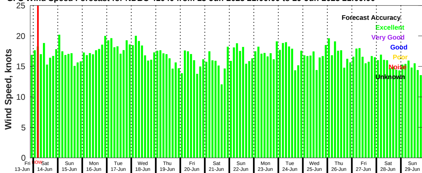
GFS Wind Speed Forecast for NDBC 41040 from 13-Jun-2025 21:00:00 to 29-Jun-2025 21:00:00
