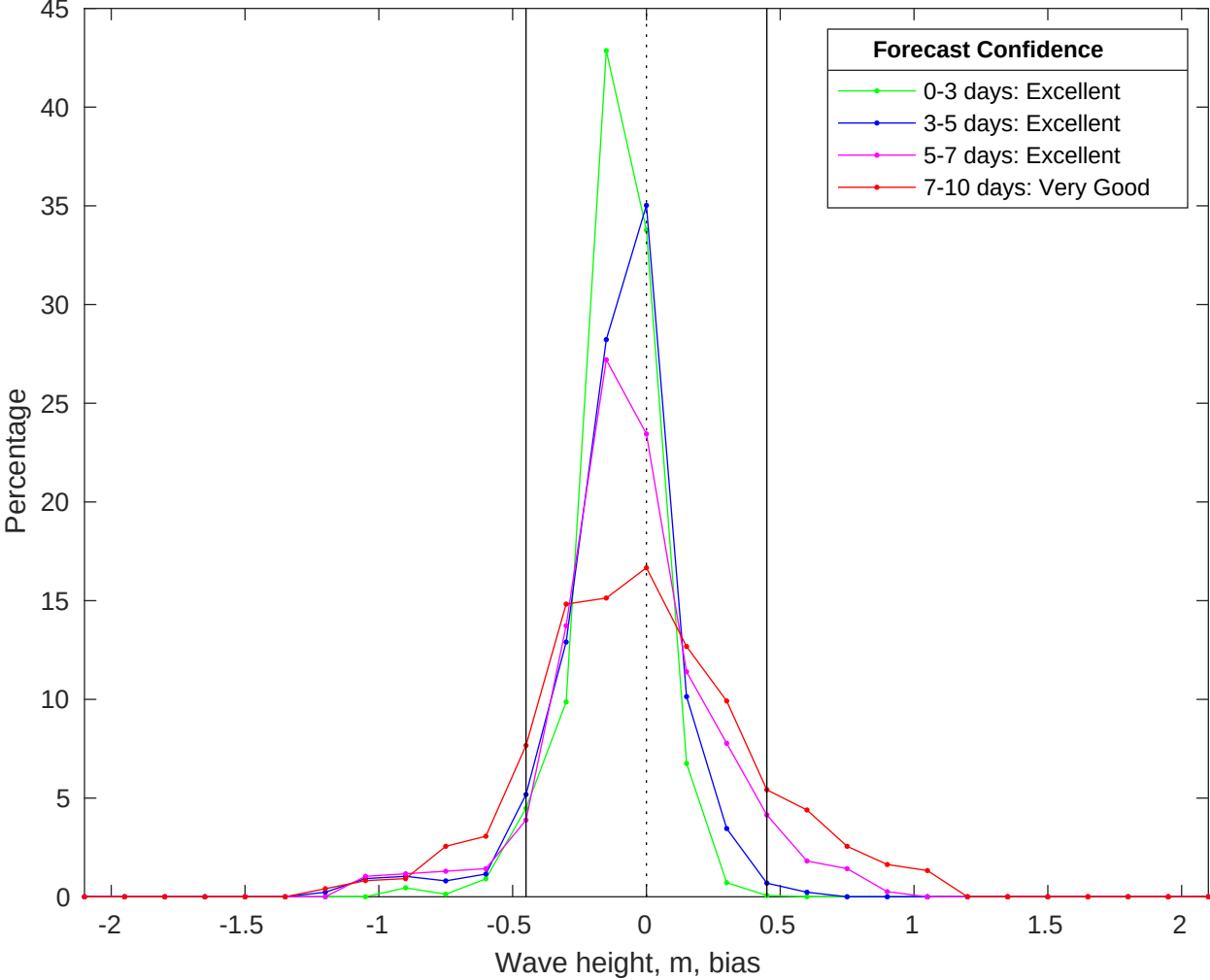
NDBC 42019 vs CMEMS Waves Bias Histogram: 14-Jun-2025
