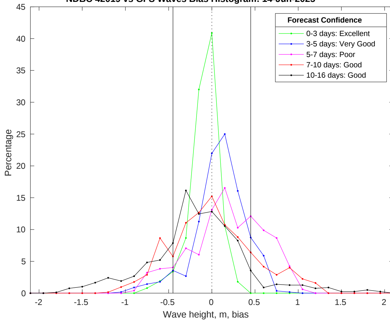
NDBC 42019 vs GFS Waves Bias Histogram: 14-Jun-2025
