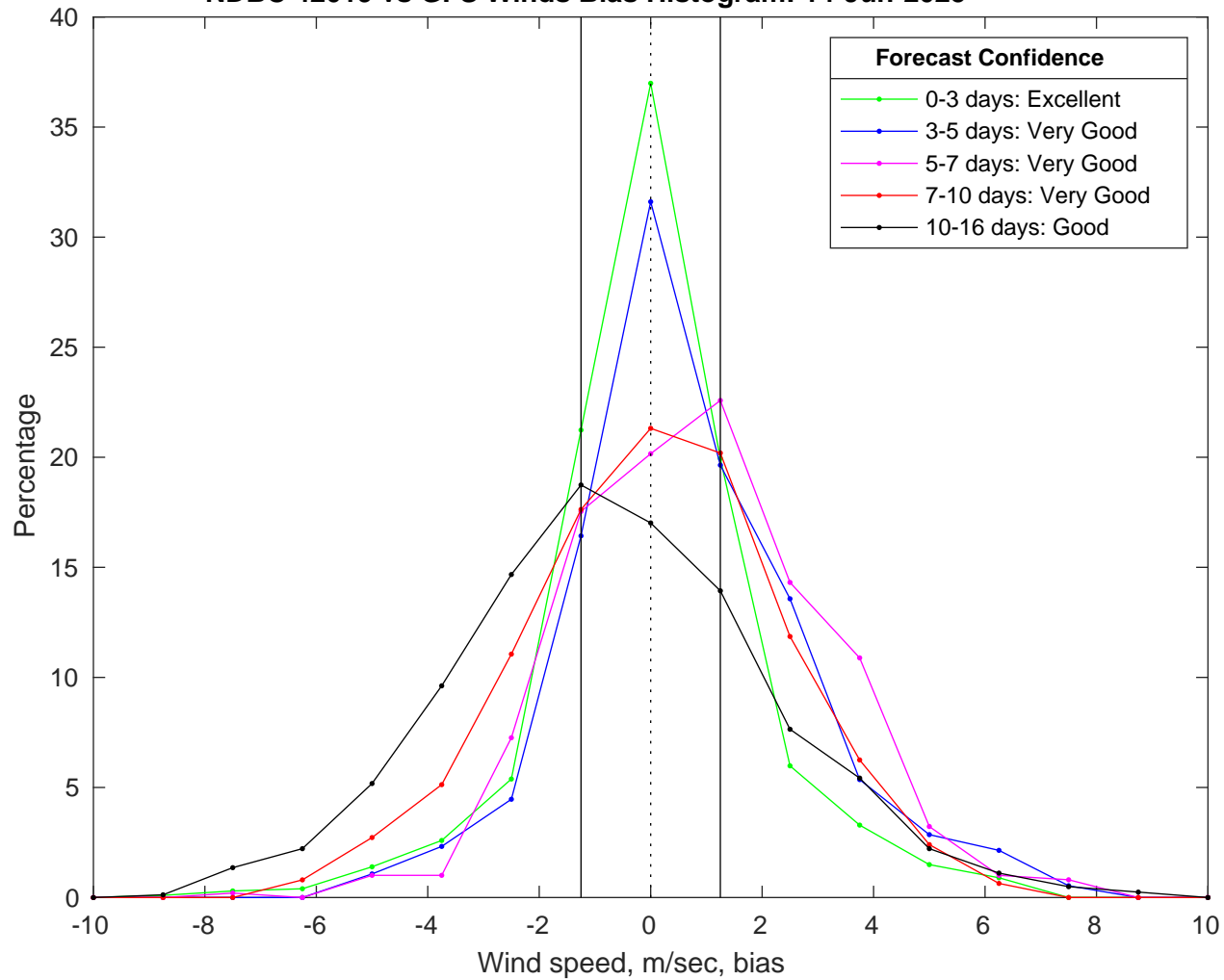
NDBC 42019 vs GFS Winds Bias Histogram: 14-Jun-2025
