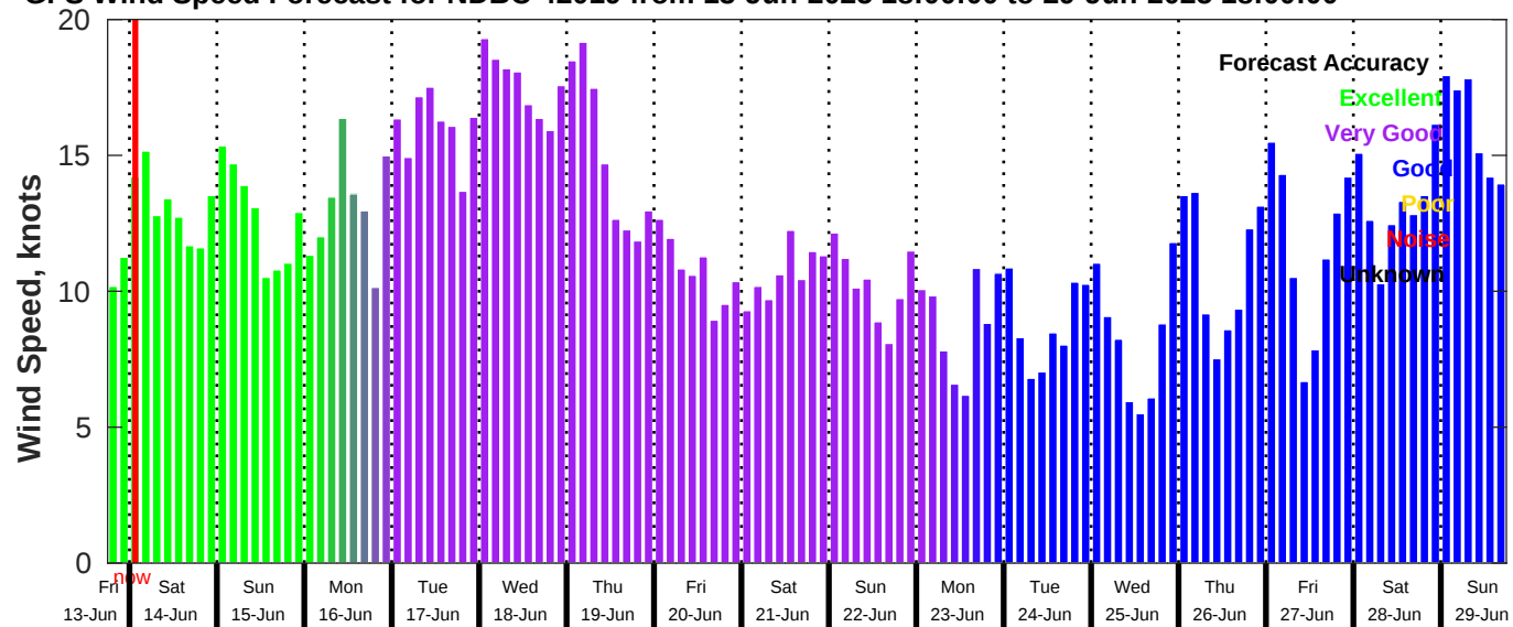
GFS Wind Speed Forecast for NDBC 42019 from 13-Jun-2025 18:00:00 to 29-Jun-2025 18:00:00
