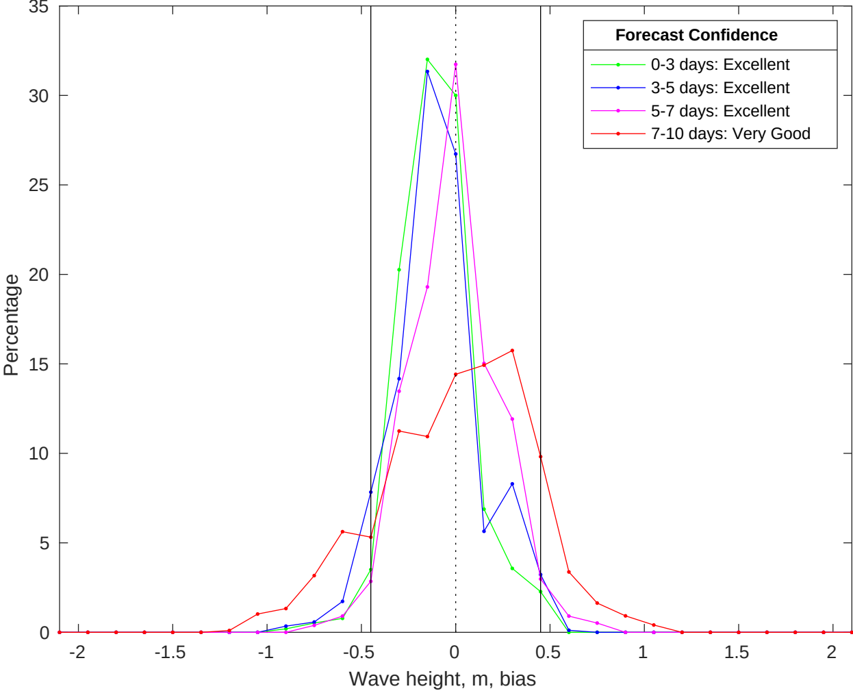
NDBC 42020 vs CMEMS Waves Bias Histogram: 14-Jun-2025
