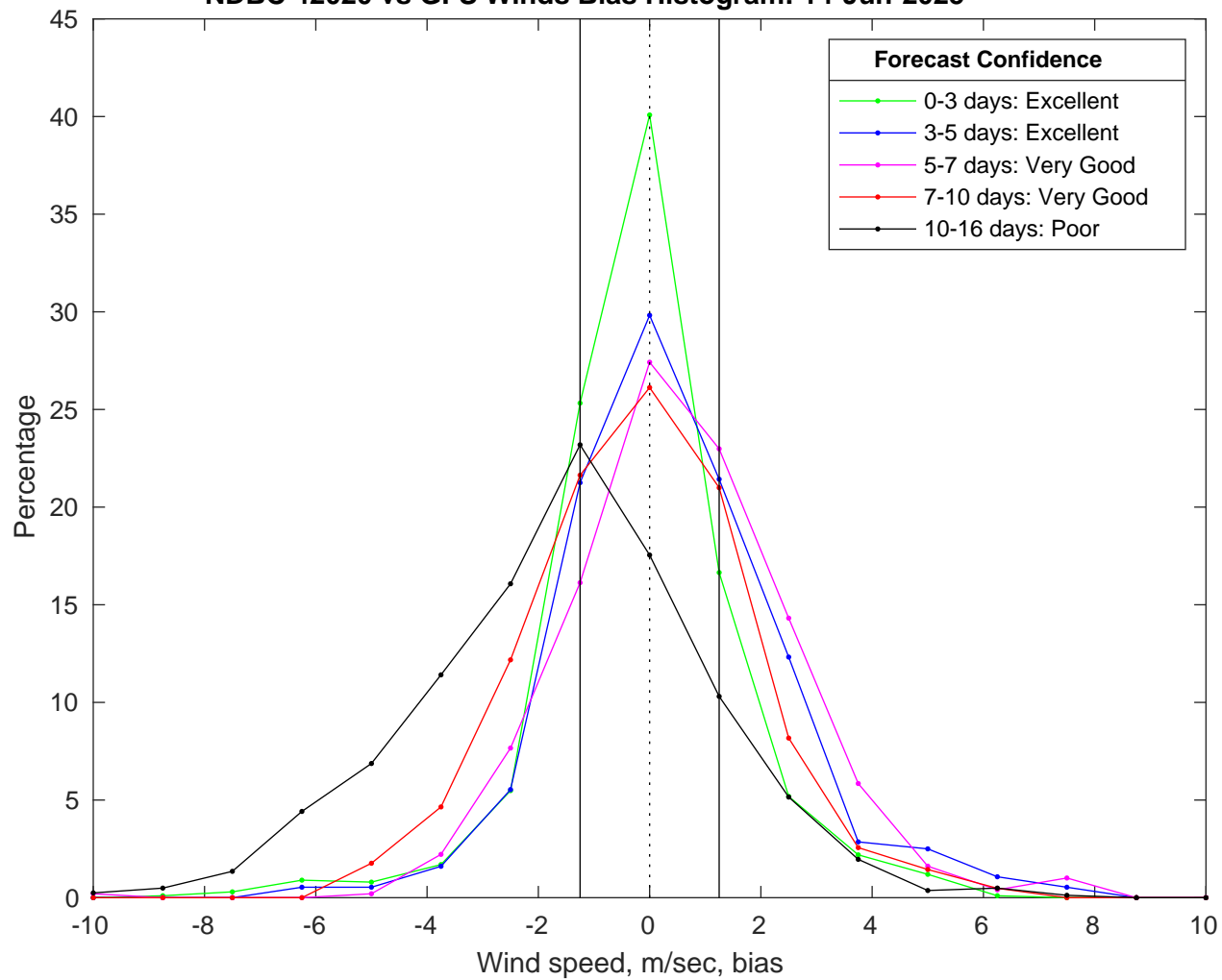
NDBC 42020 vs GFS Winds Bias Histogram: 14-Jun-2025
