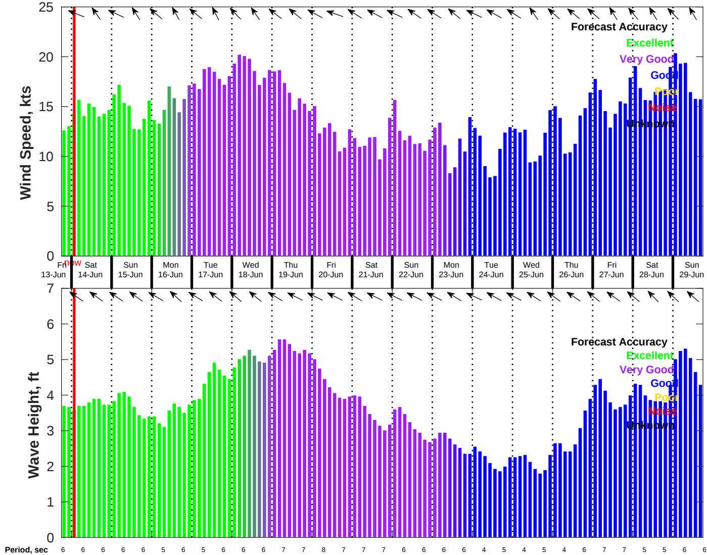
Wind & Wave Forecast for NDBC 42020 from 13-Jun-2025 18:00:00 to 29-Jun-2025 18:00:00
