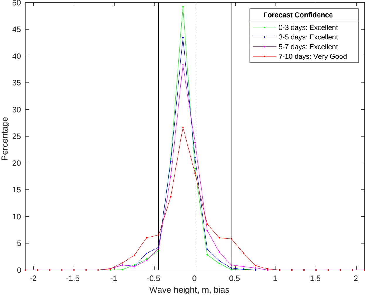
NDBC 42035 vs CMEMS Waves Bias Histogram: 14-Jun-2025
