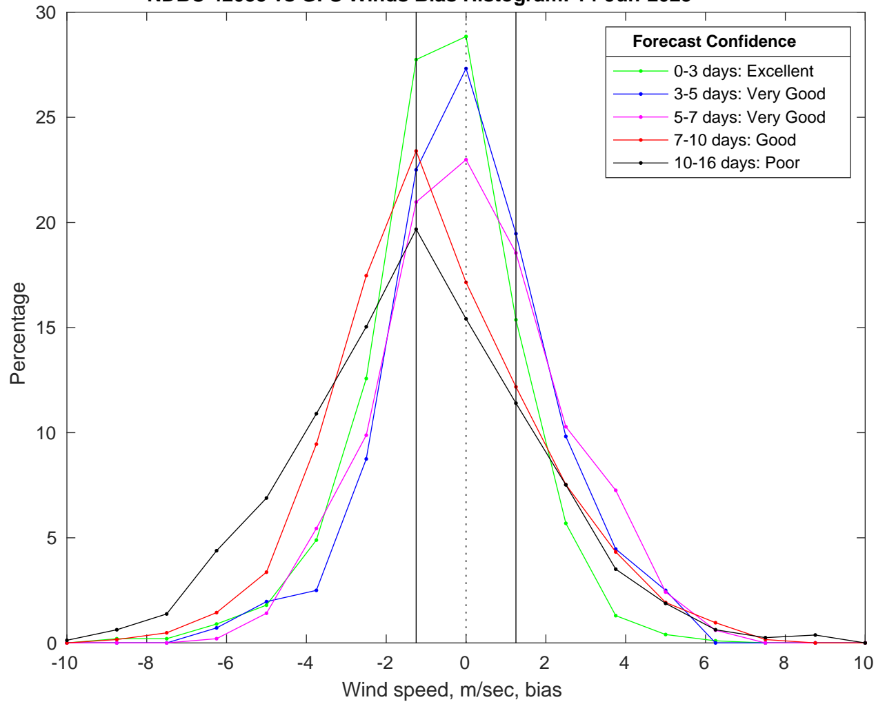
NDBC 42035 vs GFS Winds Bias Histogram: 14-Jun-2025
