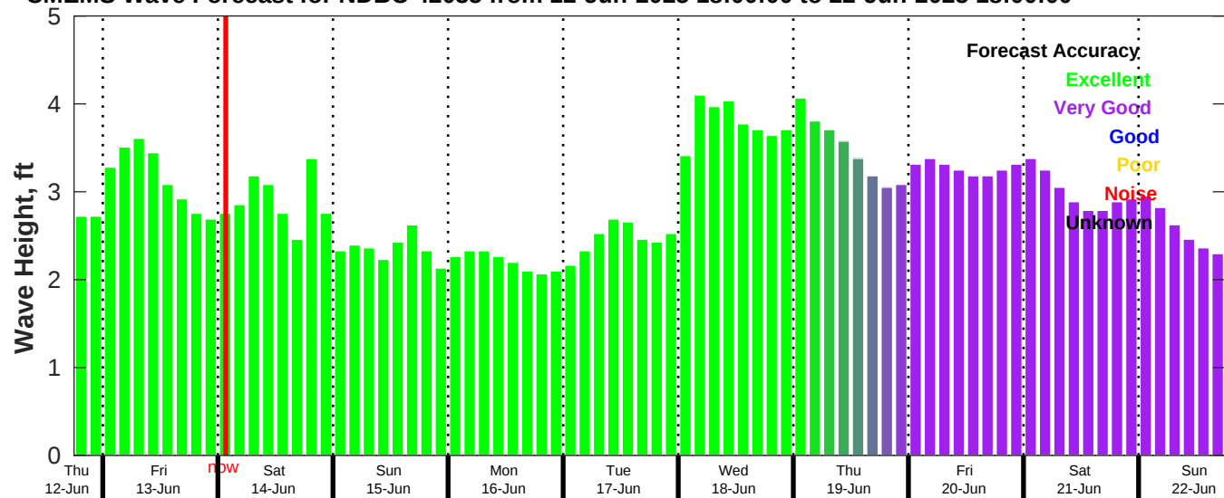
CMEMS Wave Forecast for NDBC 42035 from 12-Jun-2025 18:00:00 to 22-Jun-2025 18:00:00
