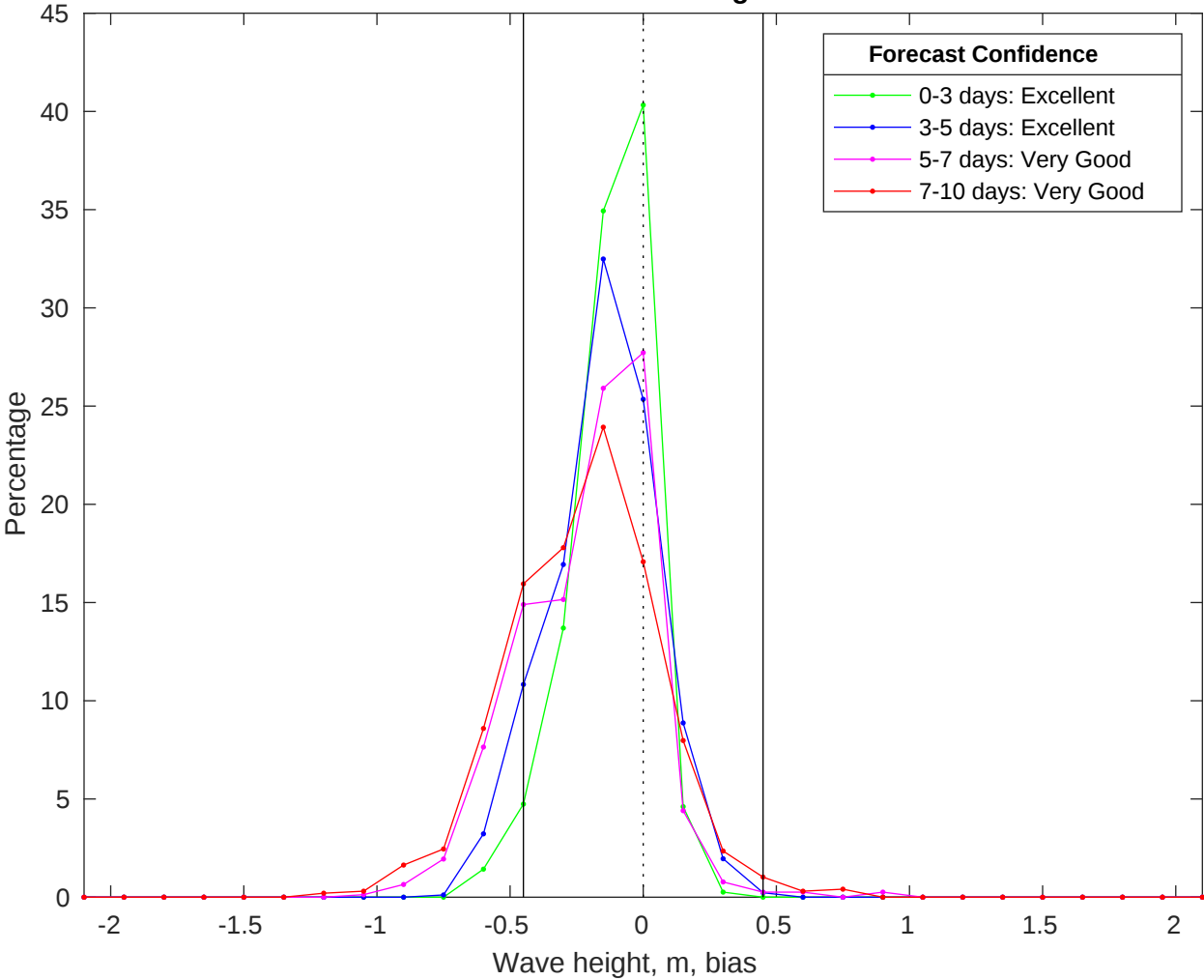
NDBC 42036 vs CMEMS Waves Bias Histogram: 14-Jun-2025
