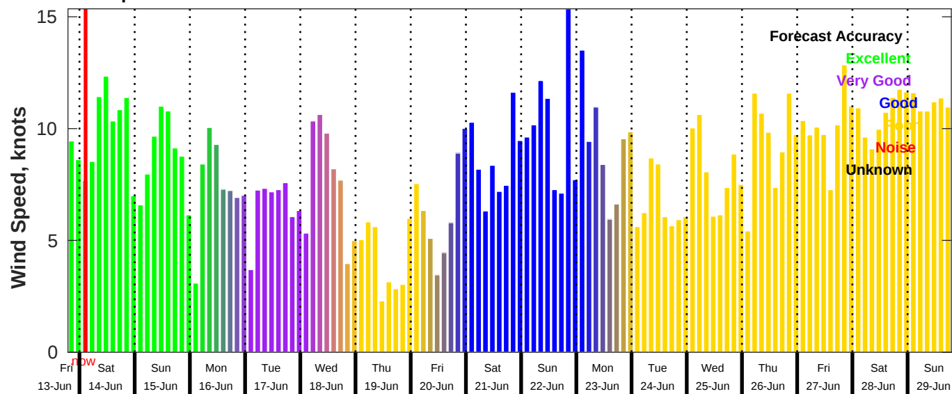
GFS Wind Speed Forecast for NDBC 42036 from 13-Jun-2025 19:00:00 to 29-Jun-2025 19:00:00
