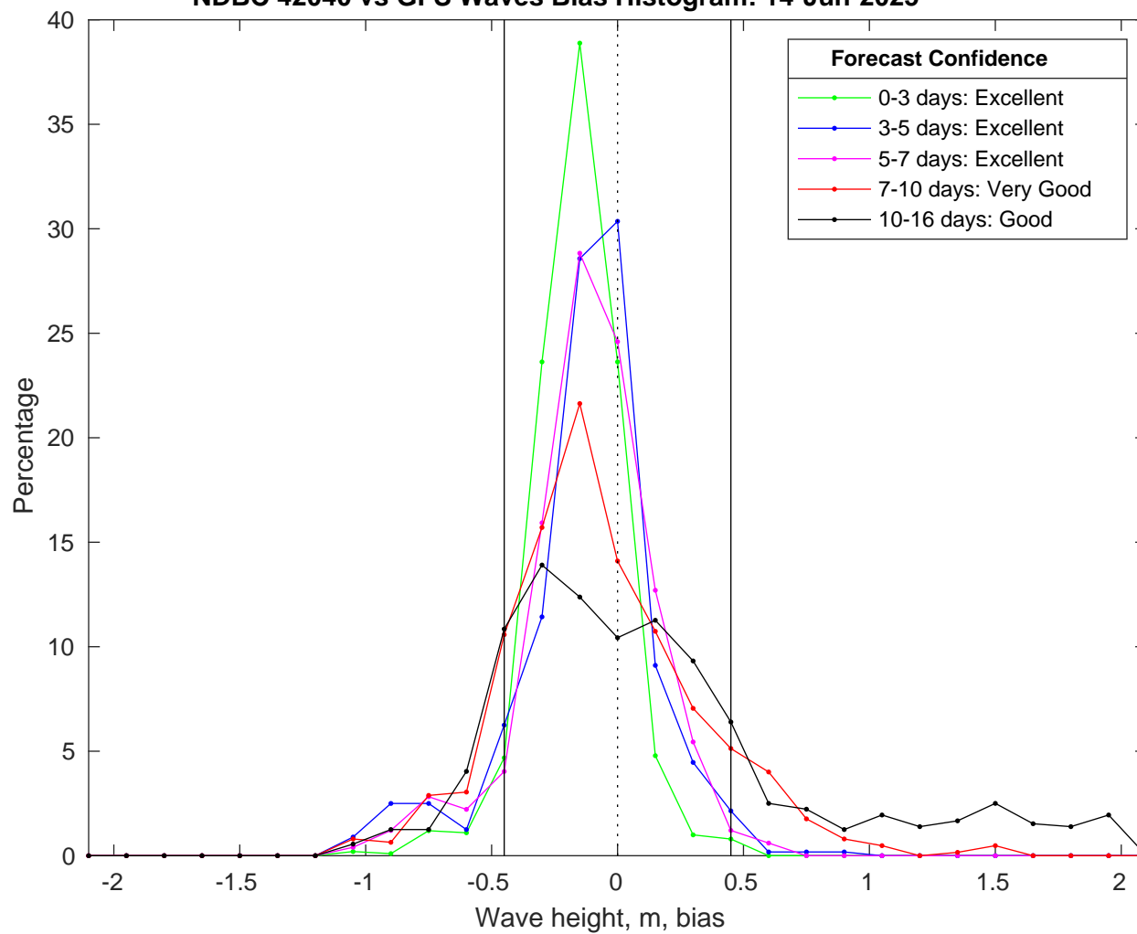
NDBC 42040 vs GFS Waves Bias Histogram: 14-Jun-2025
